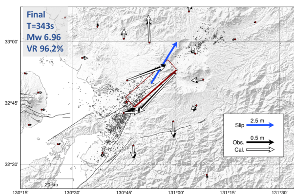
Figure 1. The real-time finite fault model for the 2016 Kumamoto Earthquake (Mw 7.0) estimated by REGARD system.
