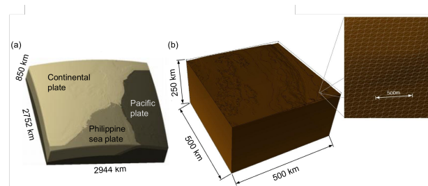
Figure 1. An example of a high-fidelity model (from Fujita et al. [2016]). (a) Macro-analysis region (0.01 Tera DOF problem with 500m resolution) (b) Micro-analysis region (2.05 Tera DOF problem with 45m resolution)
